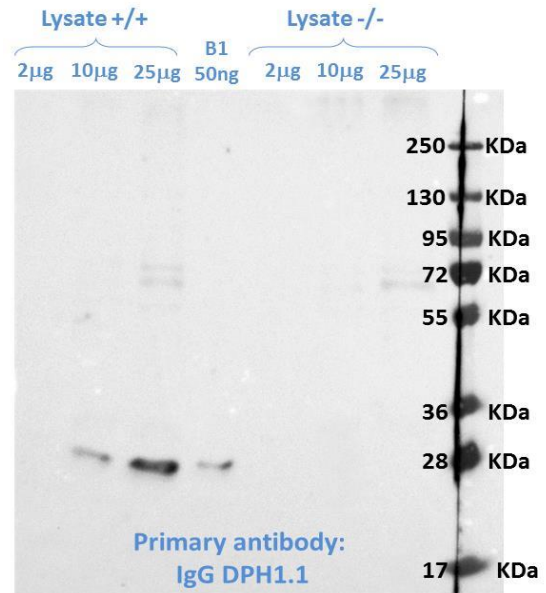
Fig. 1. Western Blot
